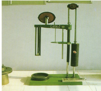
耐寒系数测定仪 cold resistant coefficient testing machine
